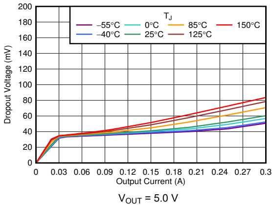
Figure 6-13. Dropout Voltage vs I_{\text{OUT}}
