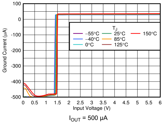
Figure 6-15. I_{\text{GND}} vs V_{\text{IN}}
