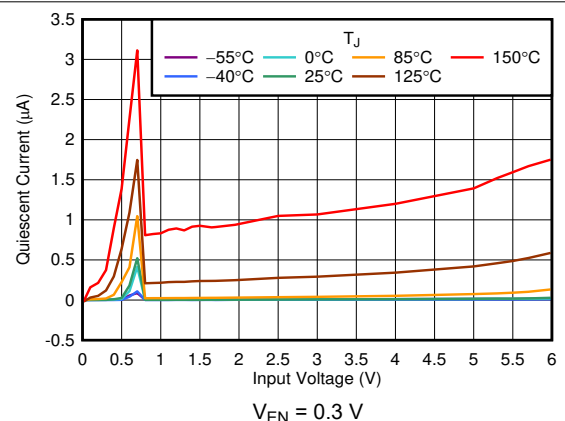
Figure 6-18. I_{\text{SHDN}} vs V_{\text{IN}}
