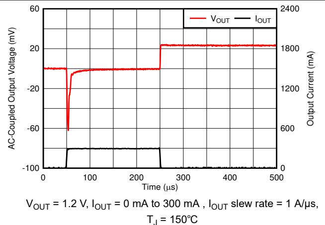
Figure 6-52. Load Transient
